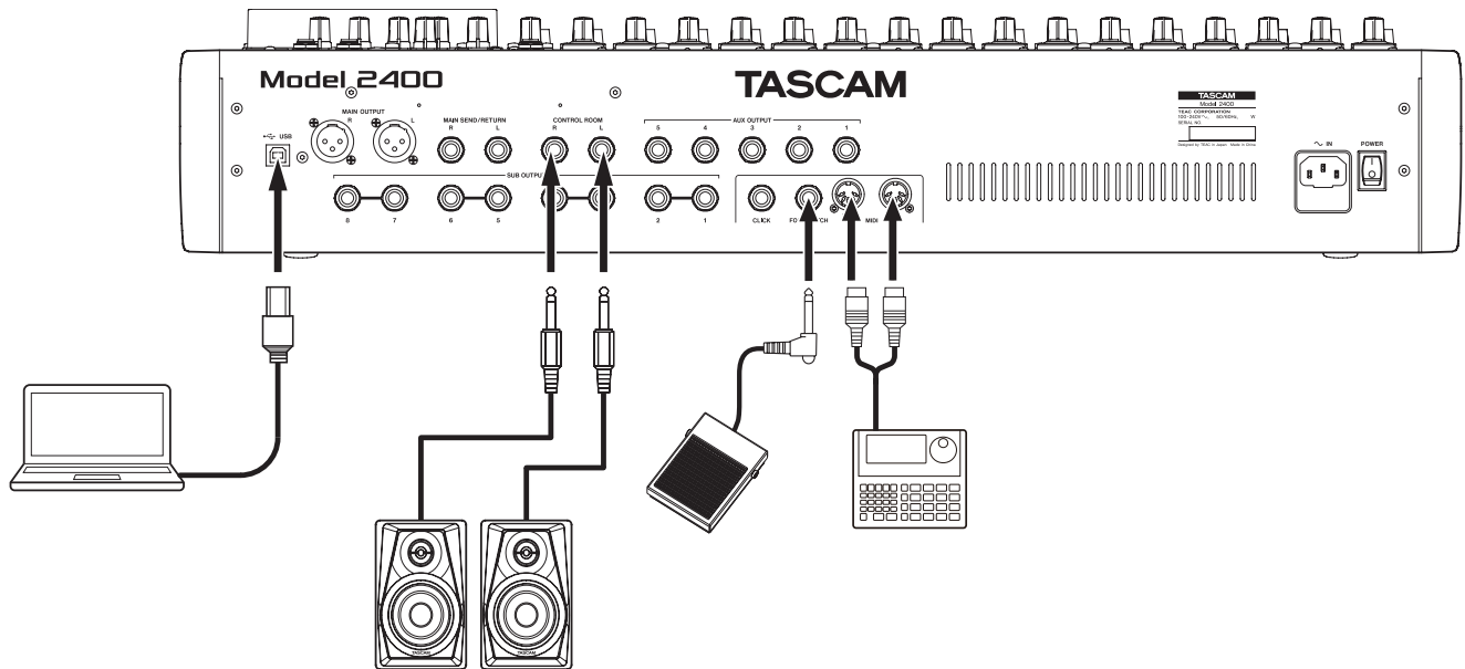
Examples of connections to a Model 2400
