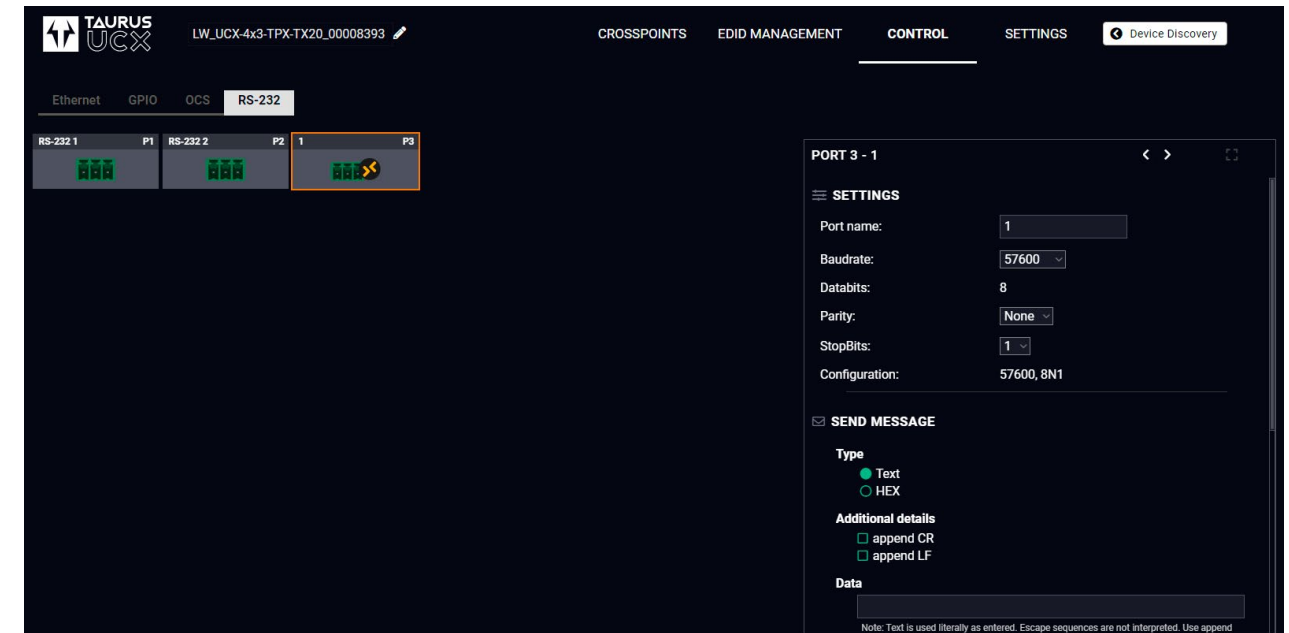
RS-232 tab in Control menu
